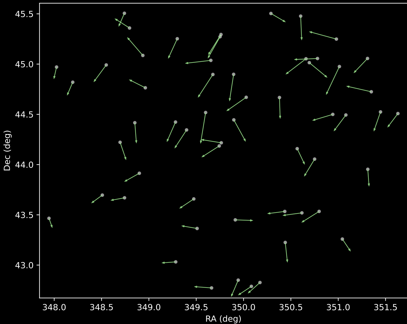
APOGEE DR17 Cluster 5 Proper Motion Vectors (n=56)
