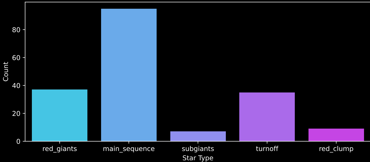
APOGEE DR17 Field: [069+42_MGA] Count plot of Star Type
