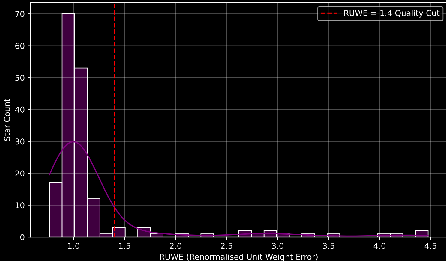
GAPOGEE DR17 Field [069+42_MGA] RUWE Distribution (n= 174)
