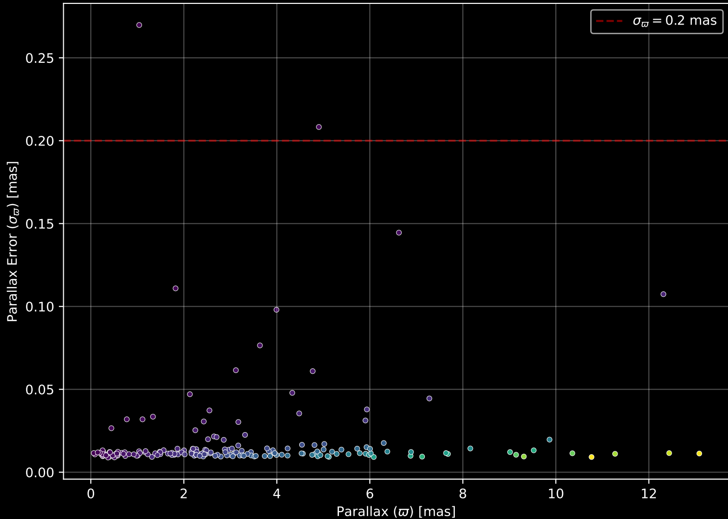
APOGEE DR17 Field: [069+42_MGA] Parallax Quality (n= 183)
