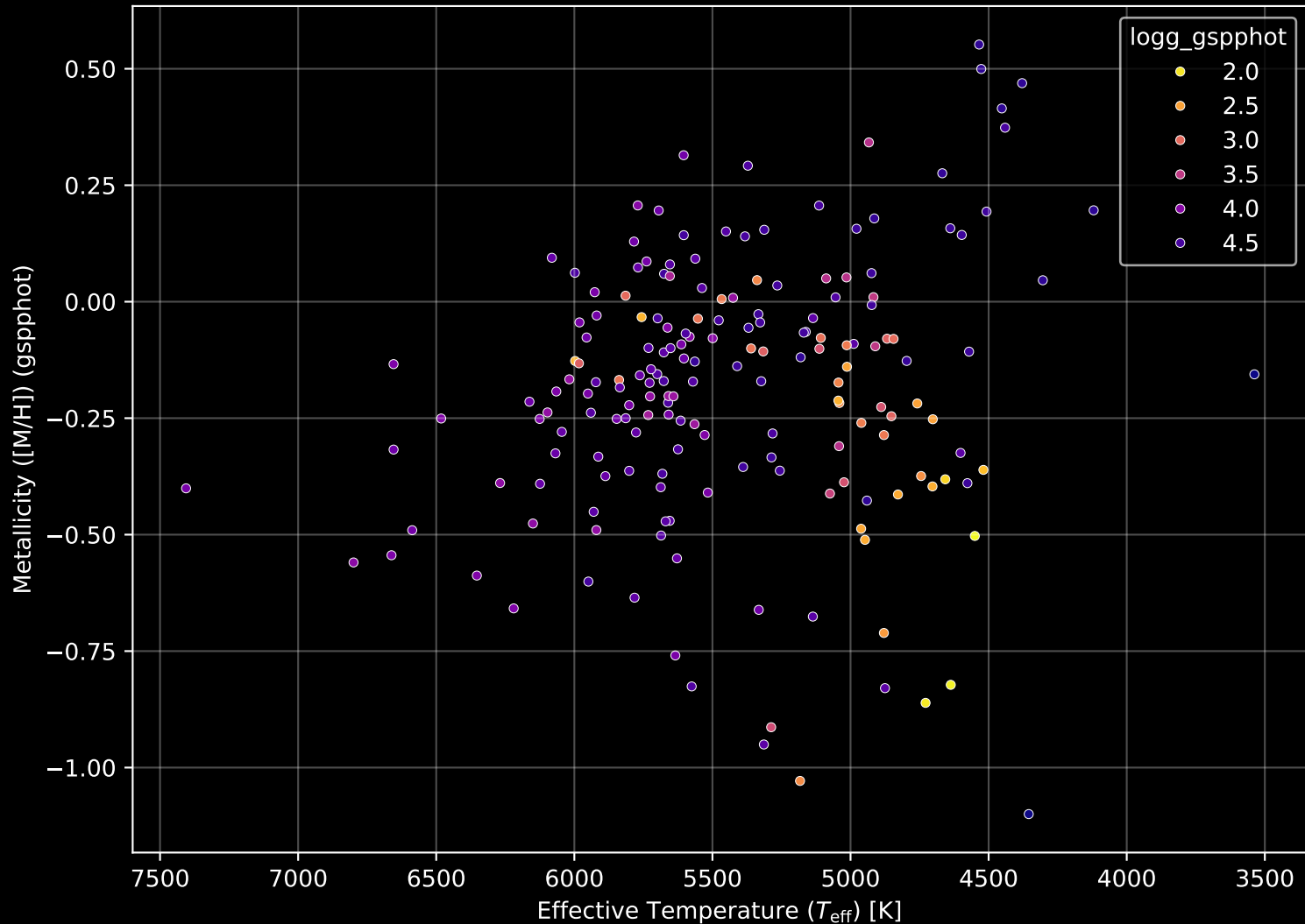
APOGEE DR17 Field: [069+42_MGA] Stellar Population Parameters (n= 183)
