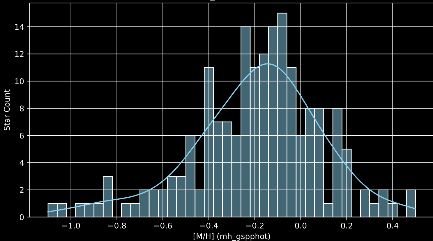
APOGEE DR17 Field: [069+42_MGA [M/H] (mh_gspphot) (n= 182)
