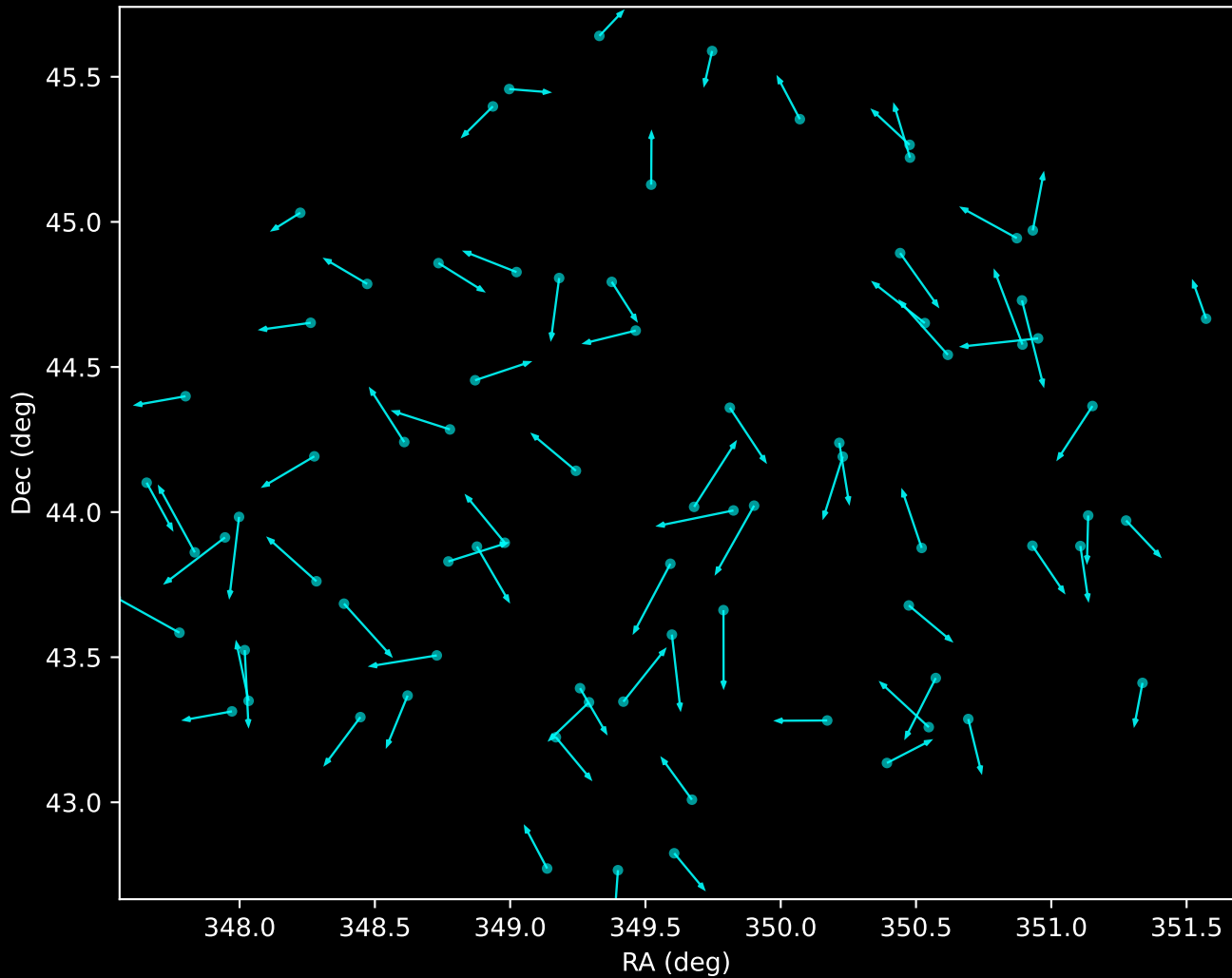
APOGEE DR17 Noise Stream Proper Motion Vectors (n=77)
