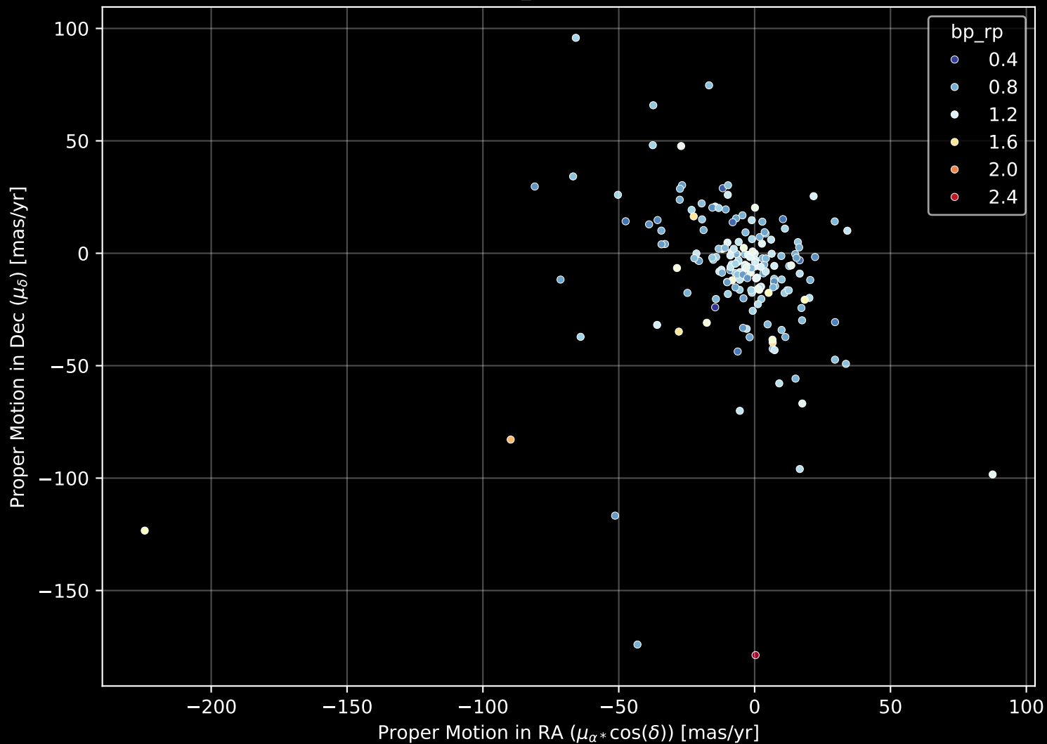
APOGEE DR17 Field: [069+42_MGA] Proper Motion Diagram (n= 183)
